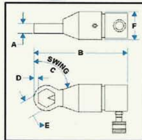
TN Nut Splitter (Model TN-105 to TN-505)
