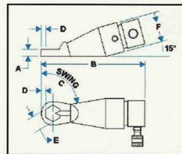
TN Nut Splitter Angle Head (Model TN-100)
